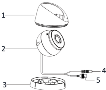
Figure 1-3 Type III/IV Turret Camera Overview
