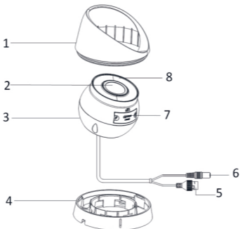
Figure 1-5 Type VI Turret Camera Overview
