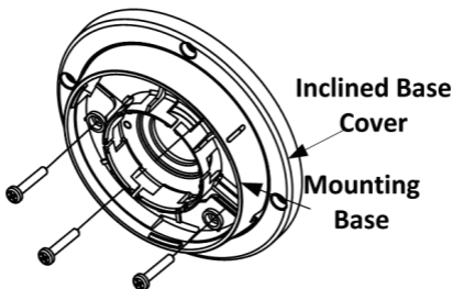
Figure 2-11 Fix Camera's Mounting Base
