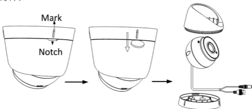
Figure 2-3 Disassemble the Camera
