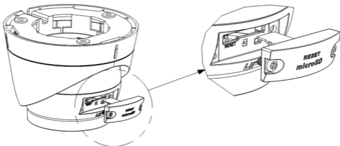
Figure 2-1 Unscrew the Cover and Insert Memory Card
