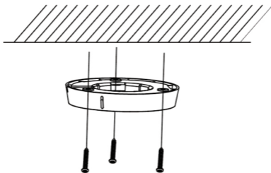
Figure 2-4 Fix the Mounting Base
