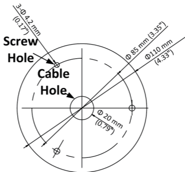
Figure 2-2 The Drill Template
