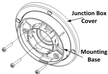
Figure 2-8 Fix screws on the junction box's Cover
