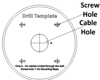
Figure 2-10 Drill Template
