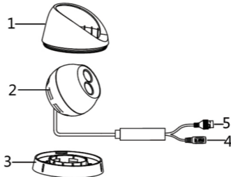
Figure 1-2 Type II Turret Camera (PoE) Overview
