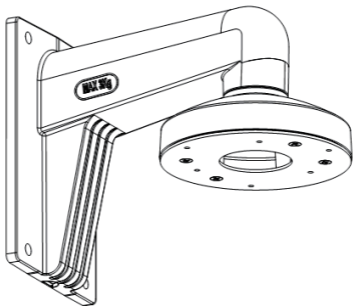
Figure 2-13 Install the Wall Mounting Bracket
