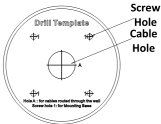
Figure 2-7 Drill Template
