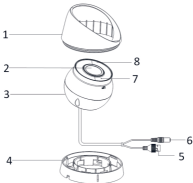
Figure 1-4 Type V Turret Camera Overview
