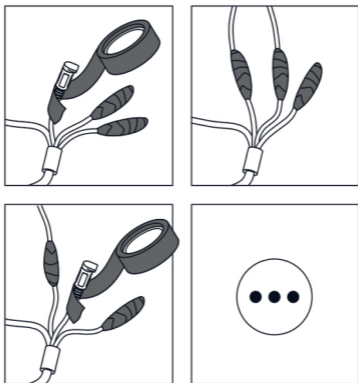
Figure 2-16 Waterproof Cables
